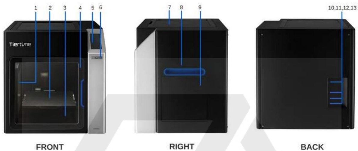
Figure 1.1 Image UP300
